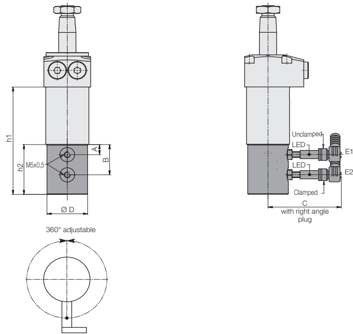
Possible position of the proximity switches
