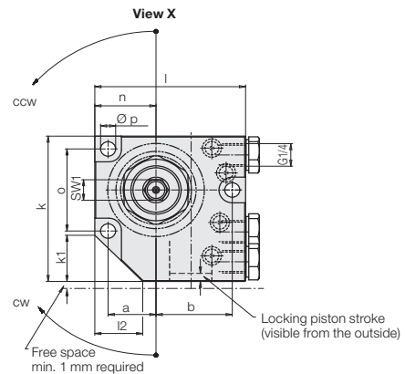
Connecting scheme
