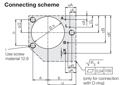
Connecting scheme
