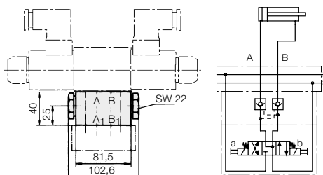
Presentation in the hydraulic circuit diagram
