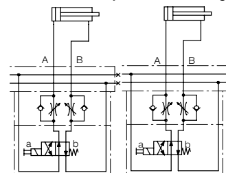
Inflow control Return-flow control
