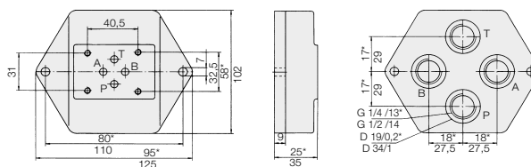
Representation 2: Connecting ports at the back
