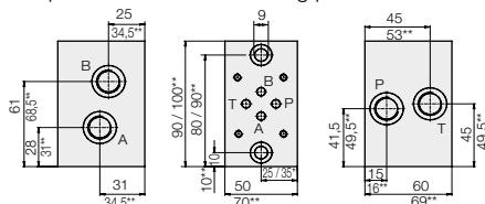
Representation 1: Connecting ports at the side
