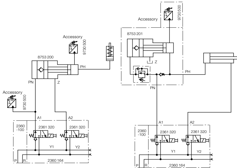
Hydraulic circuit diagram for 8753200
