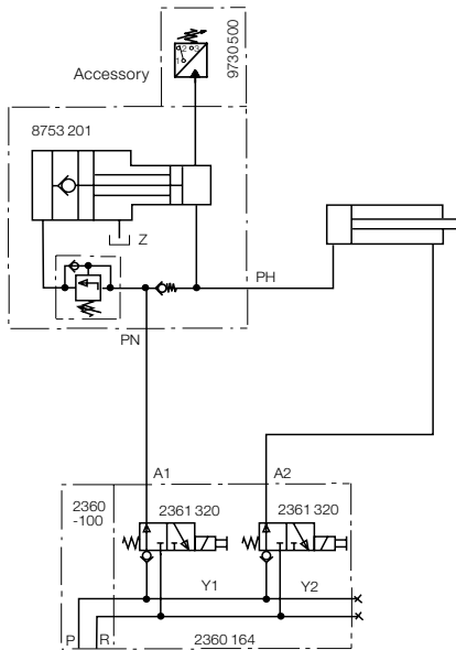
Hydraulic circuit diagram for 8753201
