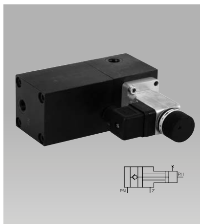
Double-acting intensifier for single-acting cylinders
