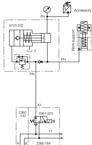
Hydraulic circuit diagram for 8753-202 / -203
