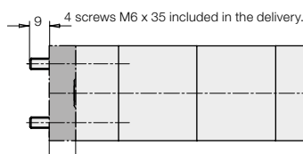
Accessory: Intermediate flange with filter screen Part no 0875500
