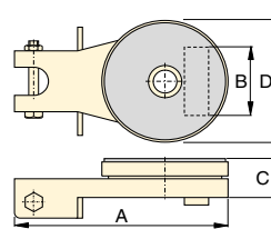
ES10, ES15, ES30 Turntable Swivel
