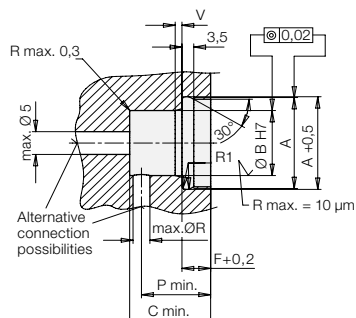
Manifold-mounting hole
