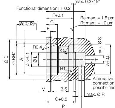
Manifold-mounting hole
