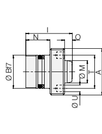
Threaded nipple
