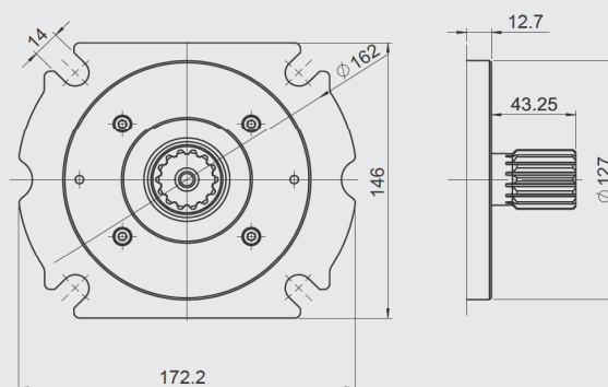
"C4" SAE C, 4-hole flange
