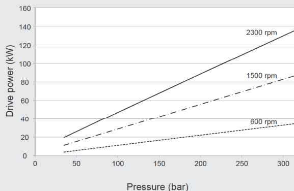
Drive power at V_{g_{max}}
