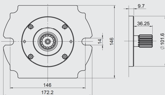
"S" SAE BB splined shaft
