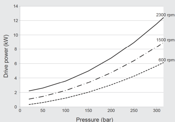
Drive power at pressure cut-off
