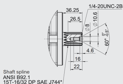
"T" SAE BB splined shaft
