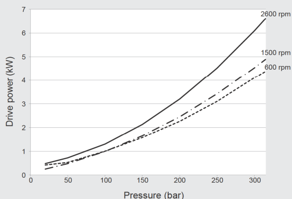
Drive power at pressure cut-off
