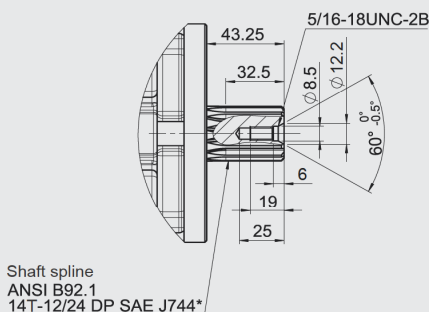
"T" SAE C splined shaft
