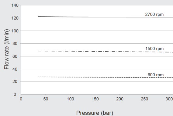
Flow rate Q_{max}
