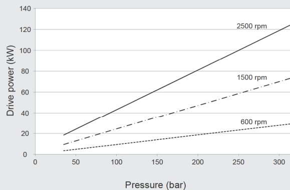
Drive power at V_{g_{max}}
