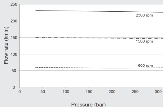
Flow rate Q_{max}
