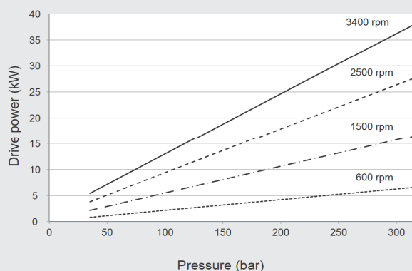
Drive power at V_{g_{max}}
