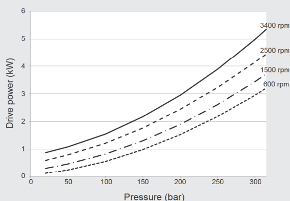
Drive power at pressure cut-off
