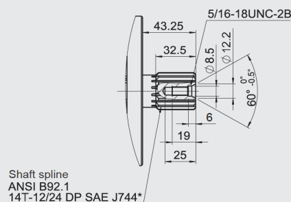
"S" SAE C splined shaft
