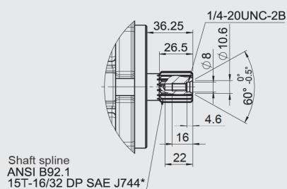
"S" SAE BB splined shaft
