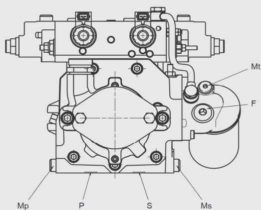
View Z
