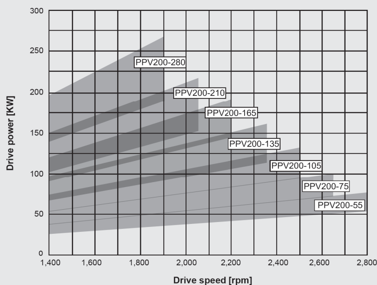
Recommended operating range, PPV200
