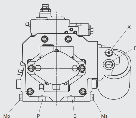
View Z
