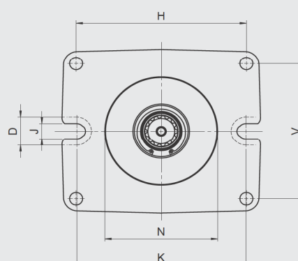
2-hole flange with 4 additional bores
