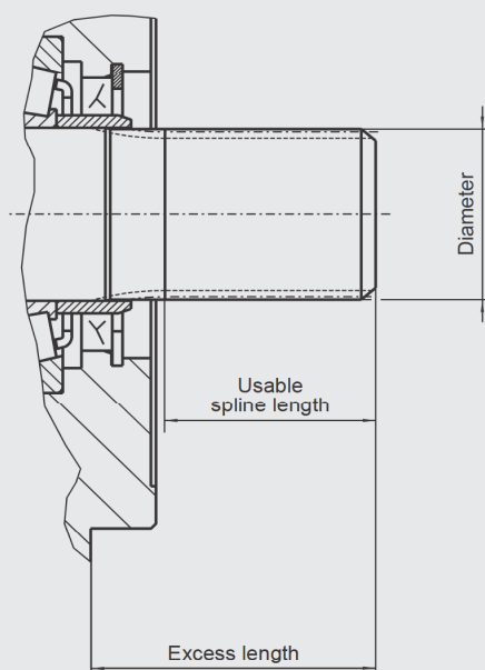
Drive shaft without undercut dimensions
