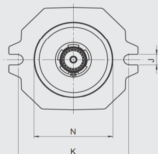
2-hole flange with 4 additional threads
