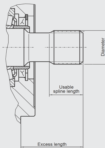
Drive shaft with undercut dimensions
