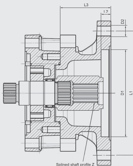
Through drive SAE - B, - B-B and -C to PGI (via intermediate flange)
