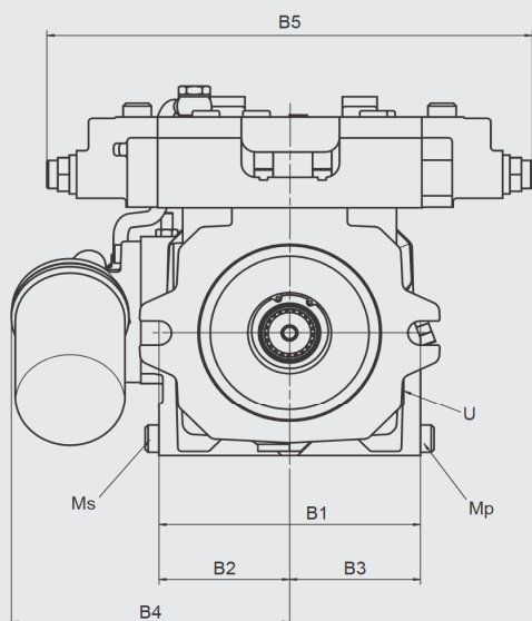
View Z
