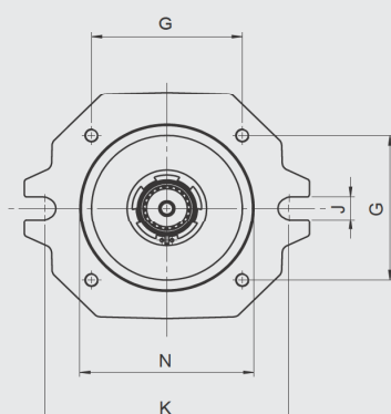
2-hole flange with 4 additional threads
