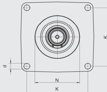
4-hole flange
