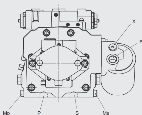
View Z
