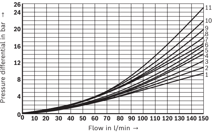
\Delta p - q_v characteristic curves
