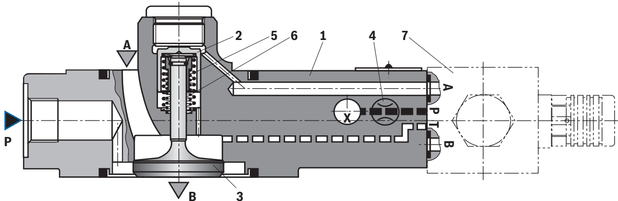
Type ZSFW... (NG32 ... 160) (without pre-decompression and built-on directional valve, vertical working direction of the control spool)
