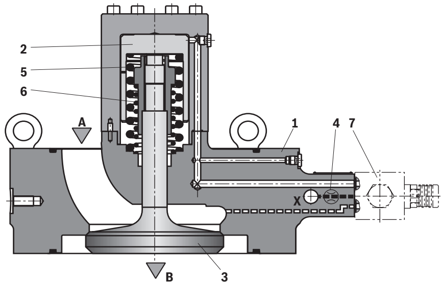
Type ZSFW... (NG200) (without pre-decompression and built-on directional valve, vertical working direction of the control spool)
