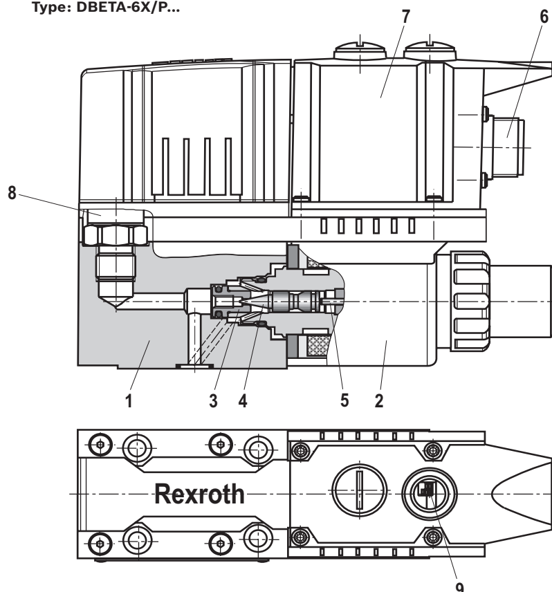
Type: DBETA-6X/P...
