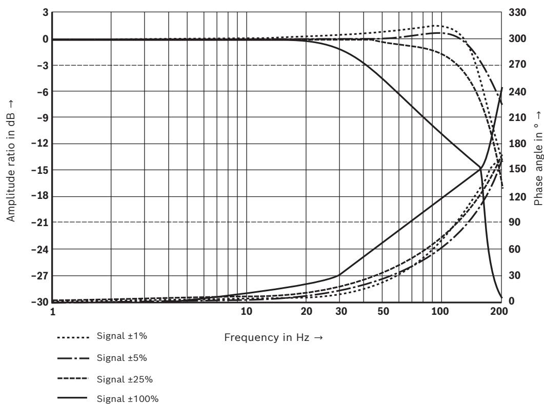
Frequency response
