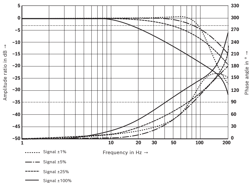
Frequency response
