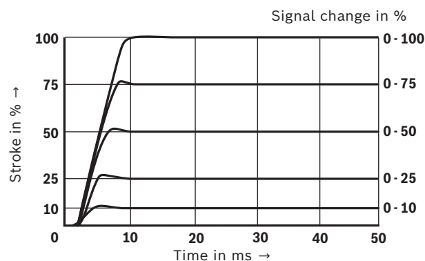
Transition function with stepped electric input signals
