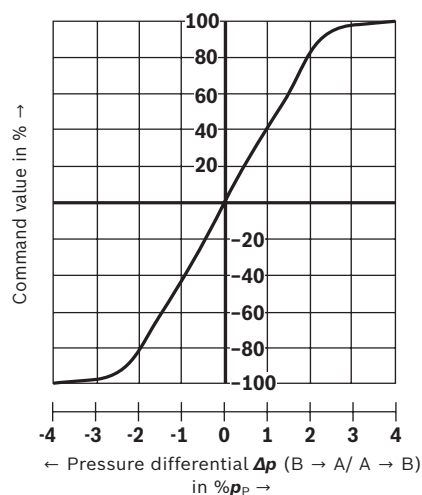
Pressure/signal characteristic curve
