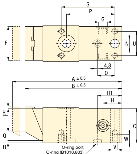
ECH-52, -202
