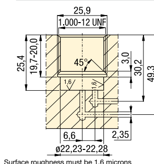
Manifold dimensions using CYDA-15 without base
