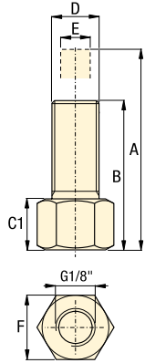
CST-2...., CST-5....
