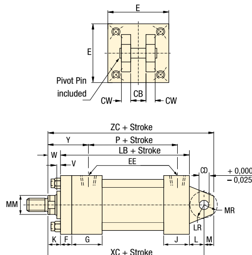
TRCM models Clevis mount
