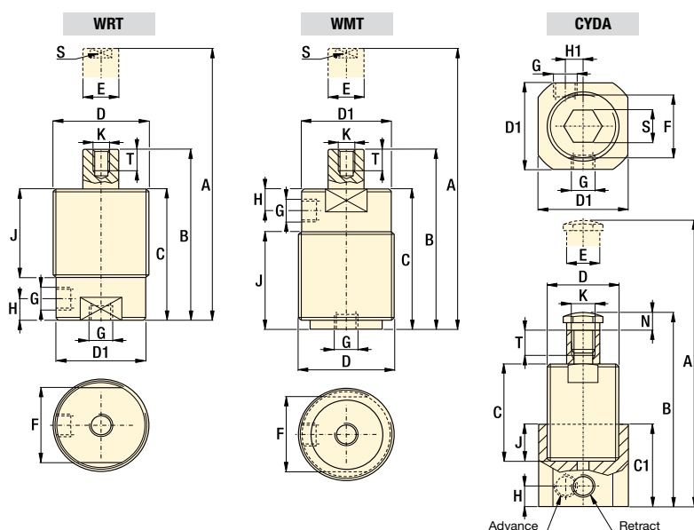
Manifold dimensions using CYDA-15 without base
