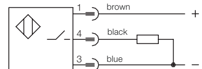
pnp (+) switching
