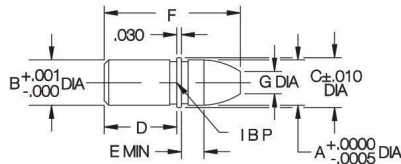
Dowel Pin
