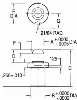
Lockscrew-Type Round Pin
