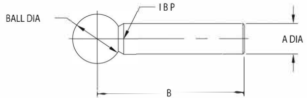
CL-00-CB 3/8" Ball
