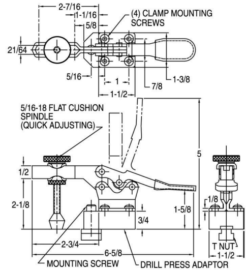
Horizontal Handle
