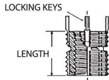
Heavy Duty – Stainless Steel Internal-Thread Locking
