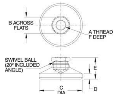
Stainless Steel with Delrin® Pad
