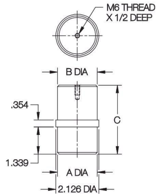
Center Pin
