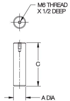
Radial Pin
