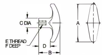
PHENOLIC — TAPPED (INCH)
