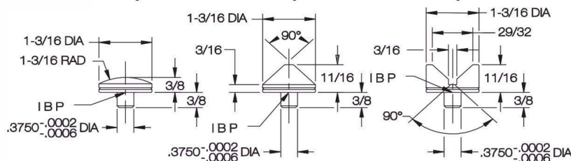
V-Shaped Tip
