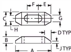
Plain Clamp
