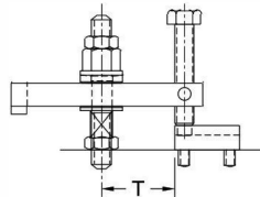
Hex-Head Clamping Screw CL-xx-THPA-HH
