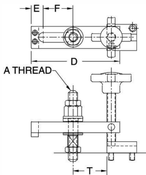
Hand-Knob Clamping Screw CL-xx-THPA-HK
