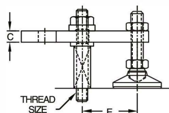
Levelling Foot CL-xxxx-2
