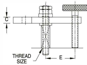
Knurled-Head Screw CL-xxxx
