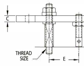
Clamp Rest CL-xxxx-1
