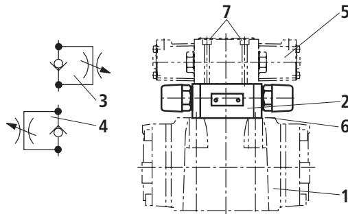
Type 4W.H 10 ..4X/...S
