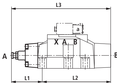
Stroke limitation on side A
