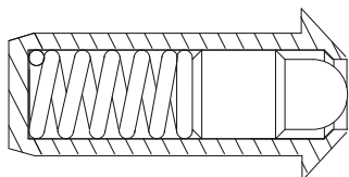
Nose Retracted
