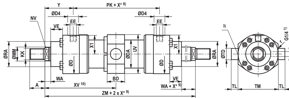
CGH1 MT4: With seal design "A", "B" and AL Ø 160 to 320 mm
