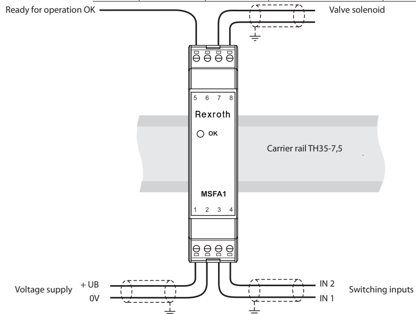
Fig. 7: Typical wiring
