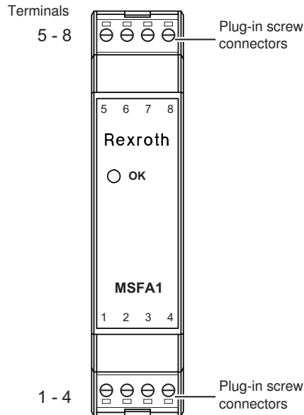
Fig. 6: Booster amplifier front view
