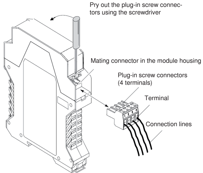
Fig. 8: Assembly/disassembly of the plug-in screw connectors
