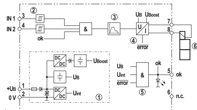
Fig. 1: Block diagram VT-MSFA1
