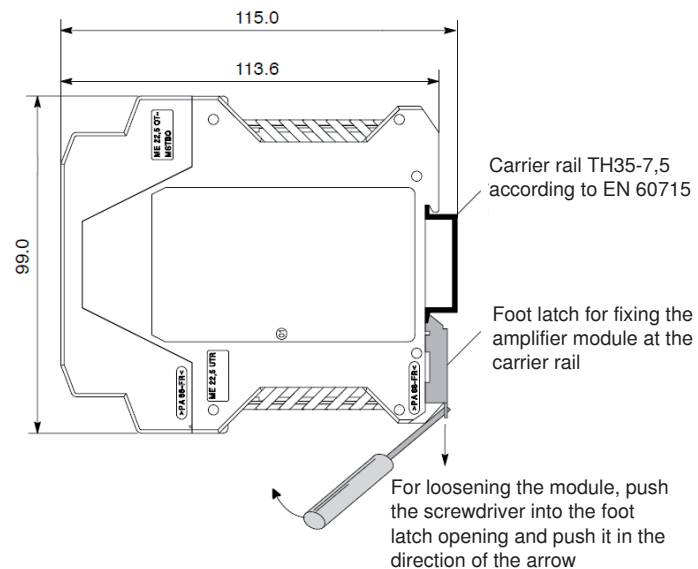
Fig. 5: Assembling/disassembling the booster amplifier
