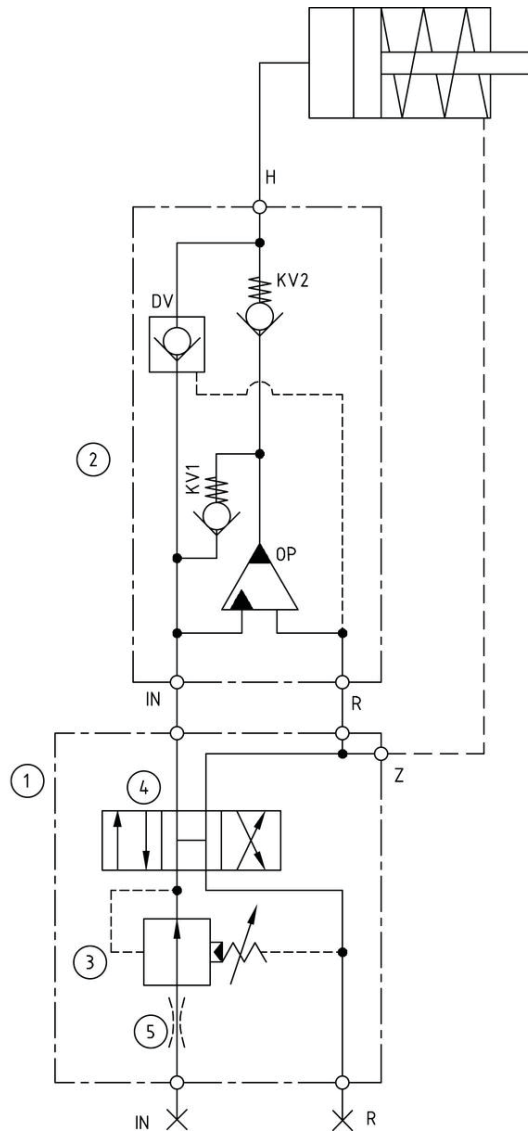
Function Diagram 1. Orifice (Optional) 2. PRV Cartridge (C10-3 Style) 3. 4/3 Cartridge (C10-4 Style) 4. Housing 5. HC2, HC4, HC7 or HC8
