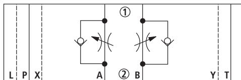
Meter-in throttling "S"
