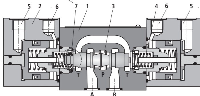
Type 4WP 6 C6X/OF/N...XC/...
