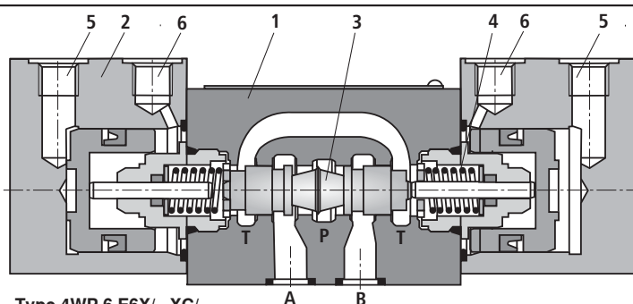
Type 4WP 6 E6X/...XC/...
