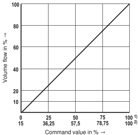
Control spool with characteristic curve L
