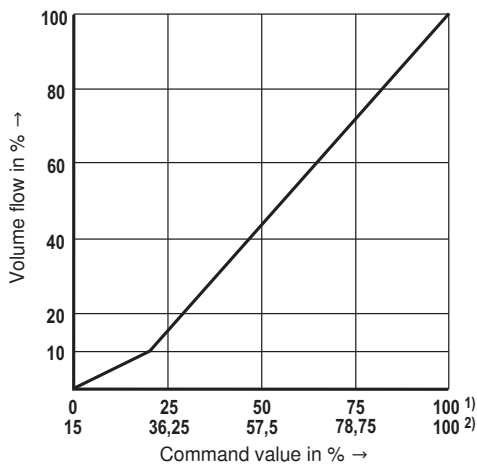
Control spool with characteristic curve P
