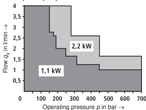
Radial piston pump
