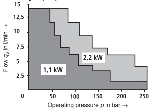
External gear pump
