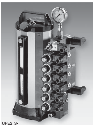
Seat valve module "S"
