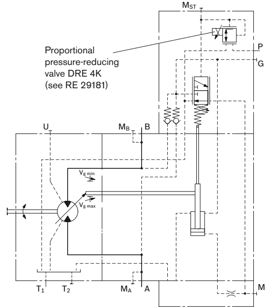
Schematic EP1, EP2 Sizes 250 to 1000
