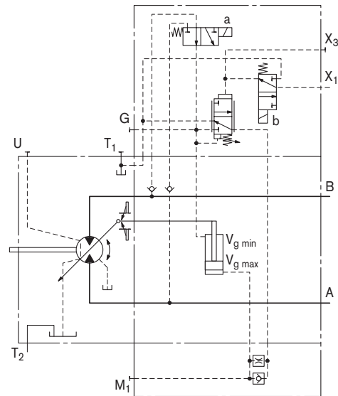
Schematic DA2, DA3, DA5, DA6 Sizes 28 to 200
