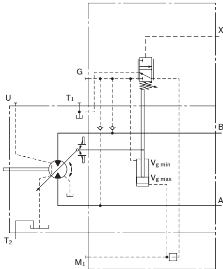
Schematic HD1, HD2, HD3 Sizes 28 to 200
