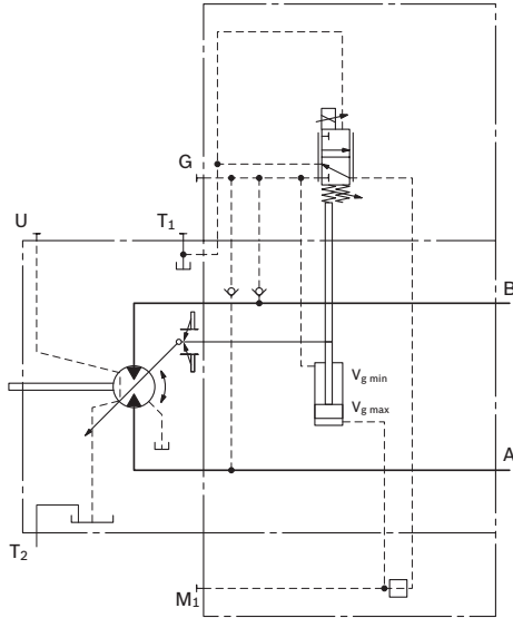
Schematic EP1, EP2 Sizes 28 to 200
