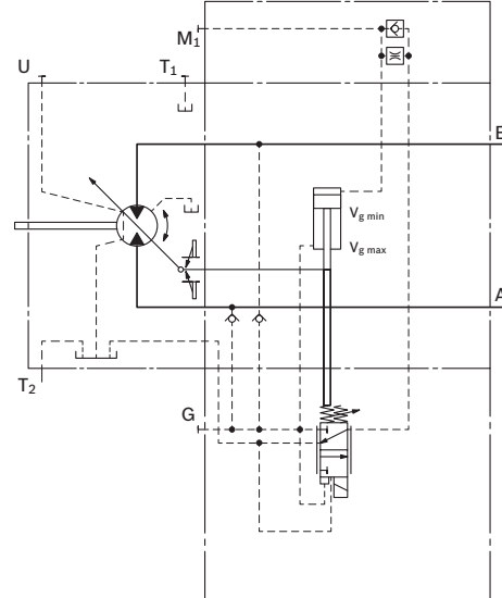
Schematic HA2U1, HA2U2
