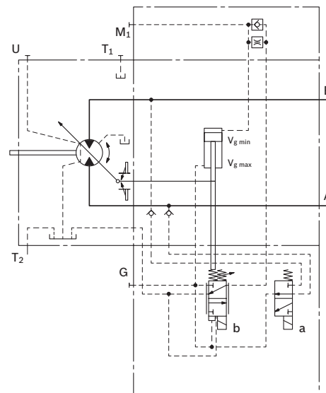
Schematic HA2R1, HA2R2
