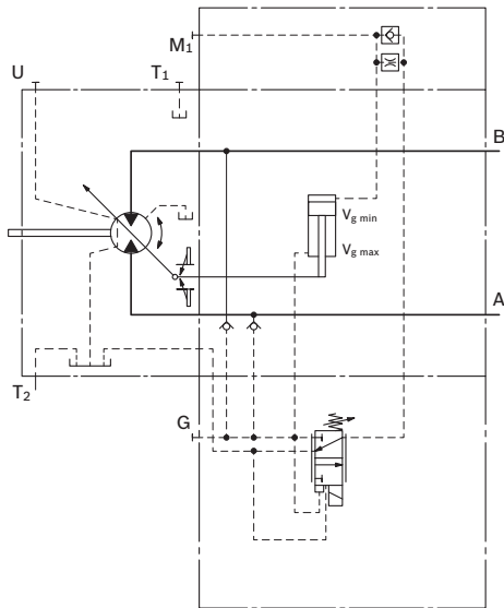
Schematic HA1U1, HA1U2
