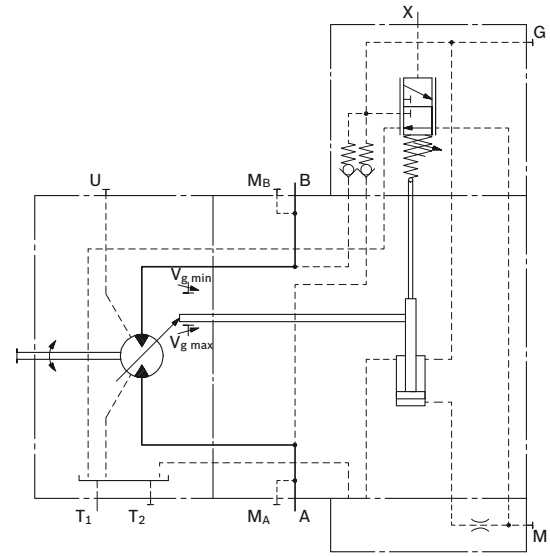
Schematic HD1, HD2, HD3 Sizes 250 to 1000
