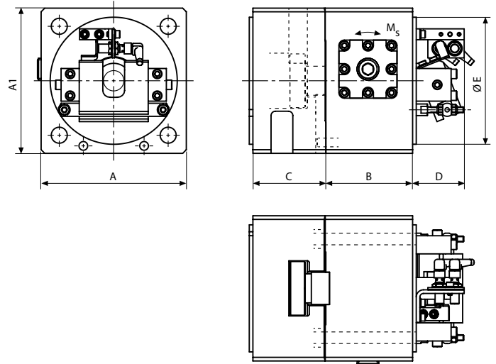
Fastening dimensions on request or according to customer's requirements
