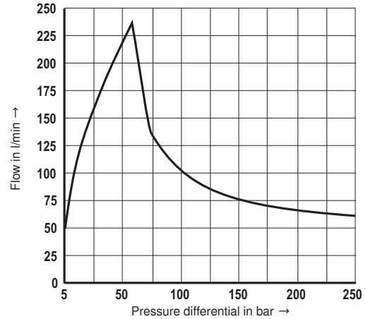
Flow characteristic curve A → T, Δp = 5 bar
