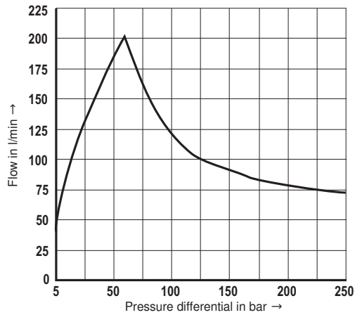
Performance limit B → T, position-controlled
