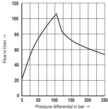
Performance limit P → A, position-controlled
