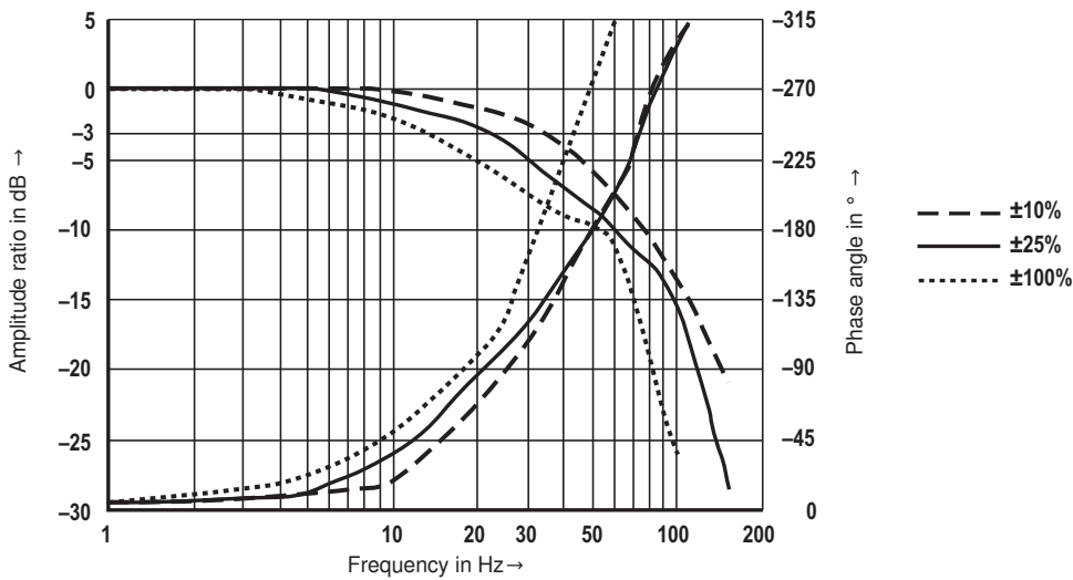
Frequency response of type STW 0196-1X/1...
