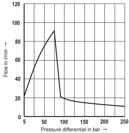
Performance limit A → T, position-controlled
