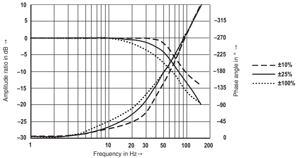
Frequency response of type STW 0195-2X/1...
