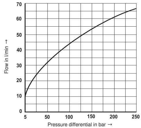
Performance limit P → A, position-controlled
