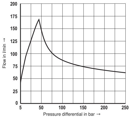
Flow characteristic curve P → A, Δp = 5 bar
