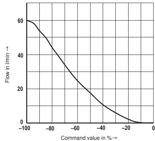
Flow characteristic curve B → T, Δp = 5 bar
