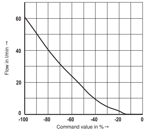
Flow characteristic curve B → T, Δp = 5 bar
