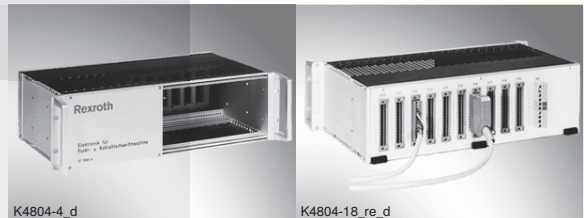
19" rack, VT 19101
