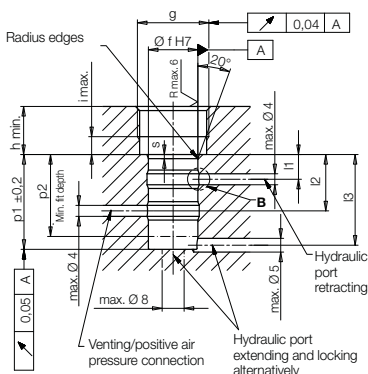
Location hole with entering slopes
