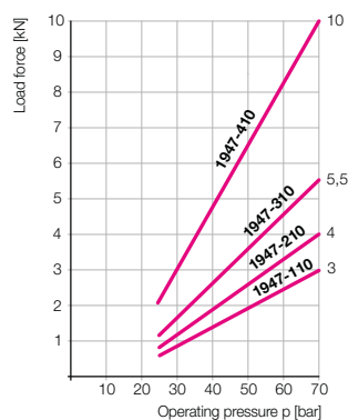
Adm. load force F As a function of the operating pressure p
