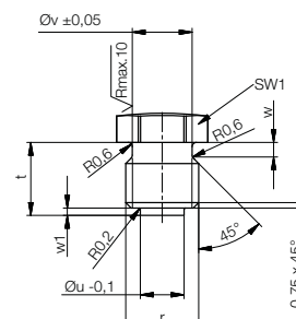
Dimensions for self-made contact bolts
