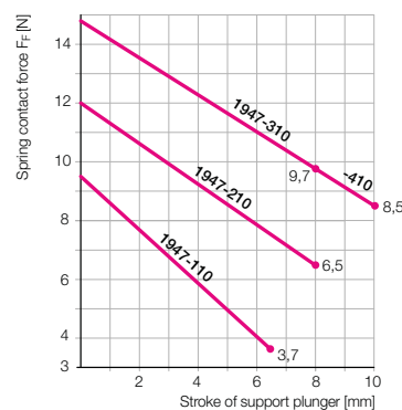
Spring contact force F F as a function of the support plunger stroke h
