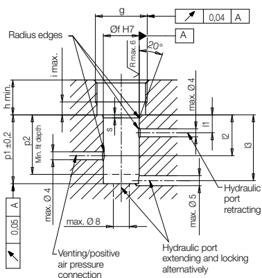
Location hole with radiused connecting bores
