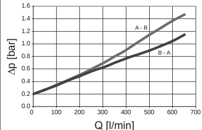
\Delta p optimized DFFX 330, 500, 660, 990, 1320
