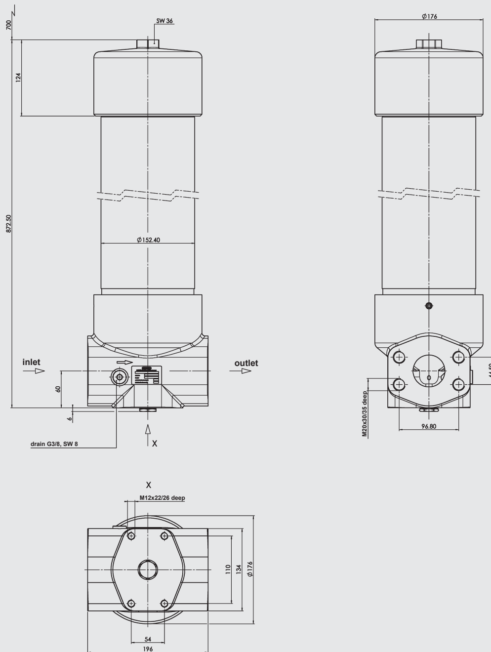
DF 1500...3.X (element top-removable)
