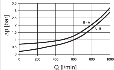
\Delta p optimized DFFX 330, 500, 660, 990, 1320
