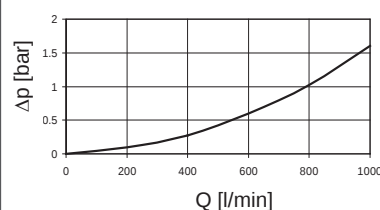
DFDK 3960 ... 3.x
