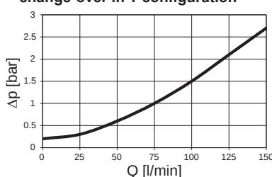
DFDK 160, 240, 280 ... 1.x with ball change-over in T configuration
