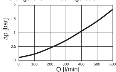
DFDK 330, 500, 660 ... 1.x DFDK 660, 990, 1320 ... 2.x with ball change-over in L configuration
