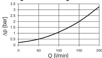
DFDK 330, 500, 660 ... 1.x DFDK 660, 990, 1320 ... 2.x with ball change-over in L configuration
