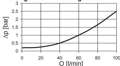
DFDK 160, 240, 280 ... 1.x with ball change-over in L configuration
