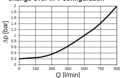
DFDK 330, 500, 660 ... 1.x DFDK 660, 990, 1320 ... 2.x with ball change-over in T configuration
