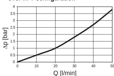
DFDK 60, 110, 140 ... 1.x with ball change-over in T configuration
