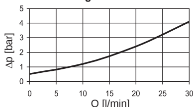
DFDK 60, 110, 140 ... 1.x with ball change-over in L configuration
