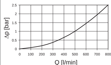
DFDK 2640 ... 3.x
