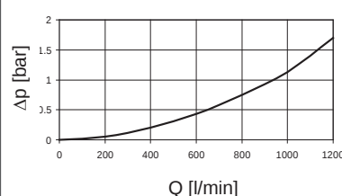
DFDK 3960 ... 3.x
