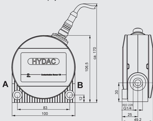
CS1x2x with display
