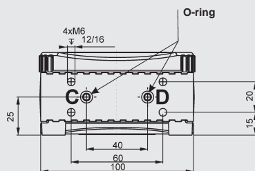
Flange connection
