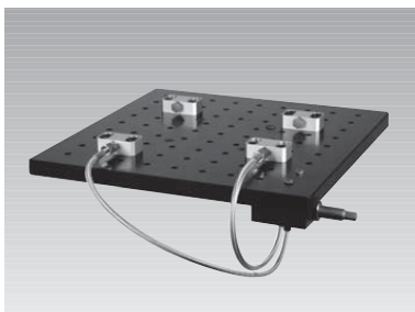
Clamping module with hydraulic clamps
