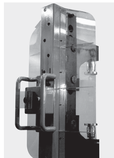
Mobile press-in frame for assembly, 80 kN basic version. Application in the handling engineering: assembly of cable control gears.
