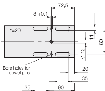
Connecting plate
