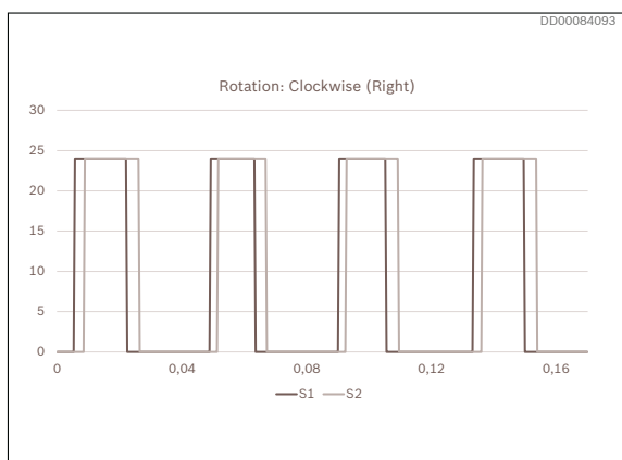
Fig. 51: Output pulses, clockwise
