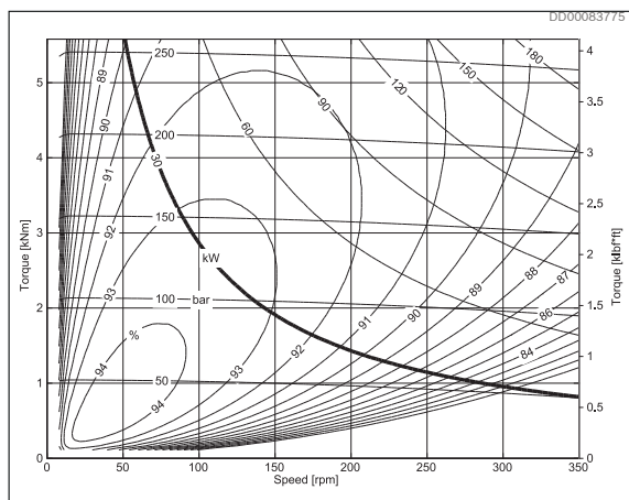
Fig. 14: CAB 20 22.5, 2 port connection
