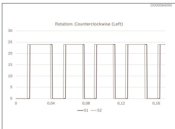
Fig. 52: Output pulses, counter clockwise
