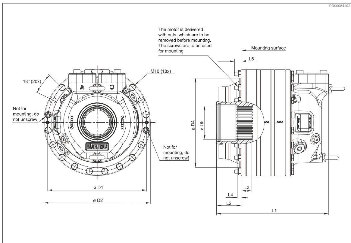
Fig. 44: CAb 30 28 F and CAb 30 30 F (front flange)
