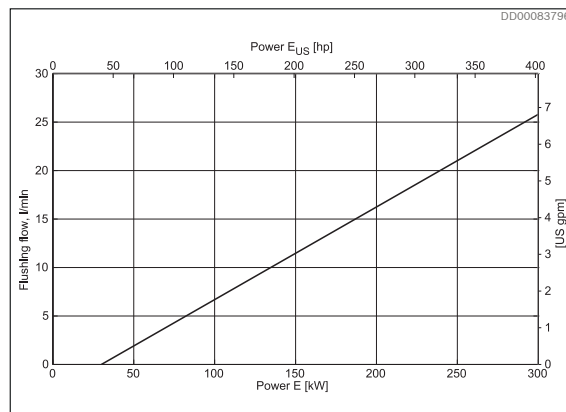
Fig. 26: Required flushing flow
