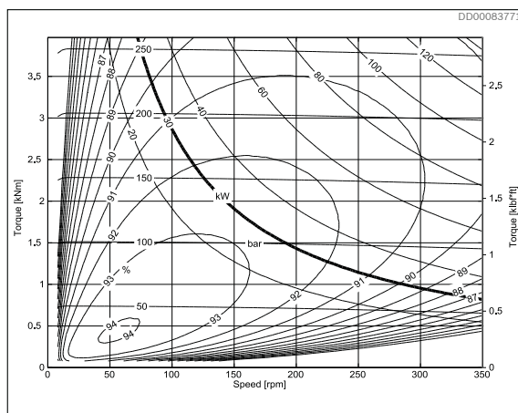
Fig. 11: CAB 20 16, 2 port connection
