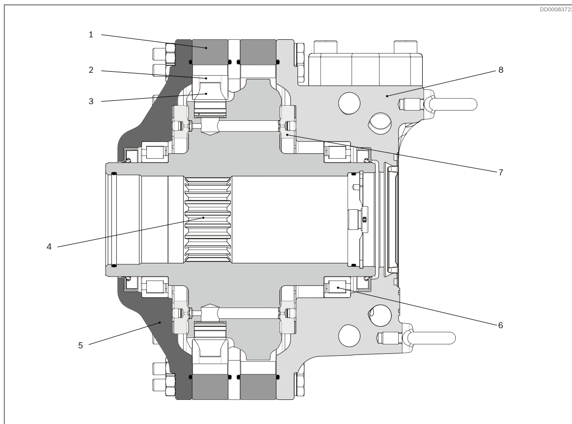
Fig. 1: Section view of radial piston hydraulic motor
