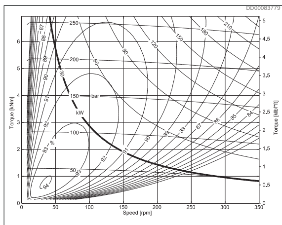
Fig. 16: CAB 30 28, 2 port connection
