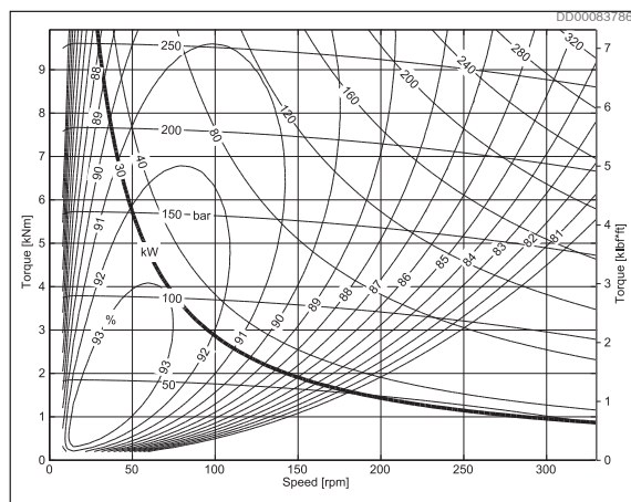
Fig. 21: CAb 40 40, 2 port connection
