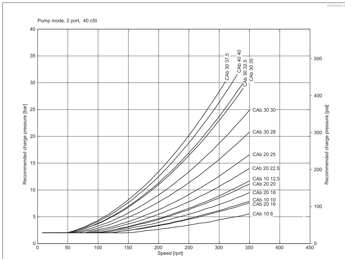
Fig. 6: Recommended charge pressure for motor working in braking mode, Häggblunds CAb 2-port connection. Valid for oil viscosity 40 cSt.
