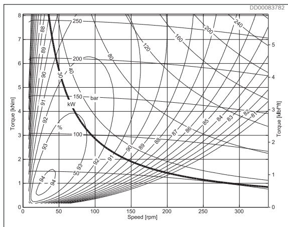
Fig. 18: CAb 30 32.5, 2 port connection
