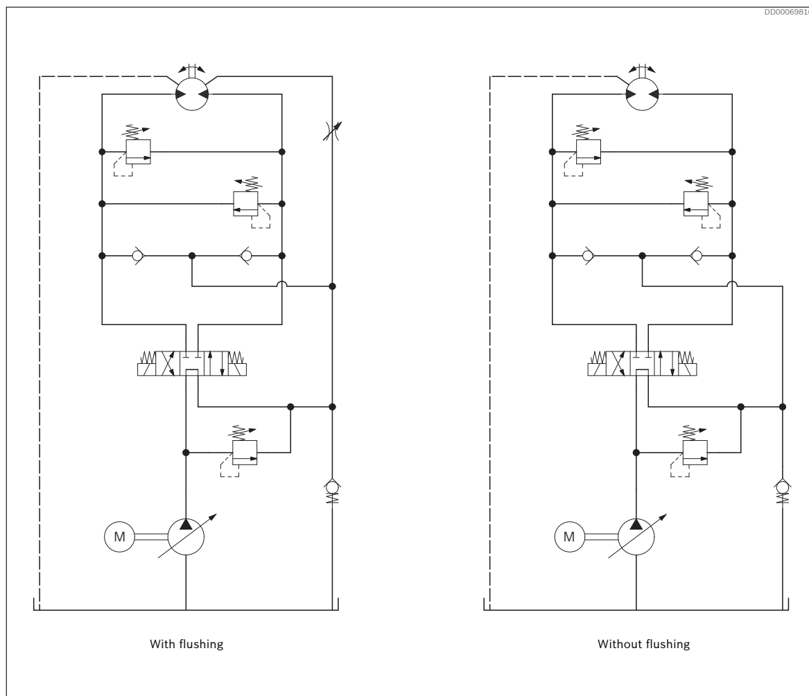
Fig. 54: Simplified open circuit design example
