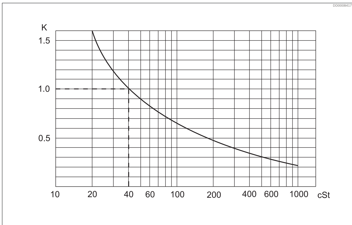
Fig. 29: Viscosity factor K
