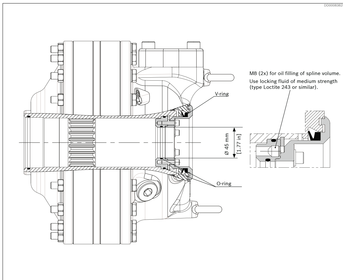
Fig. 41: Example: Hägglunds CAb 20 with through hole kit.
