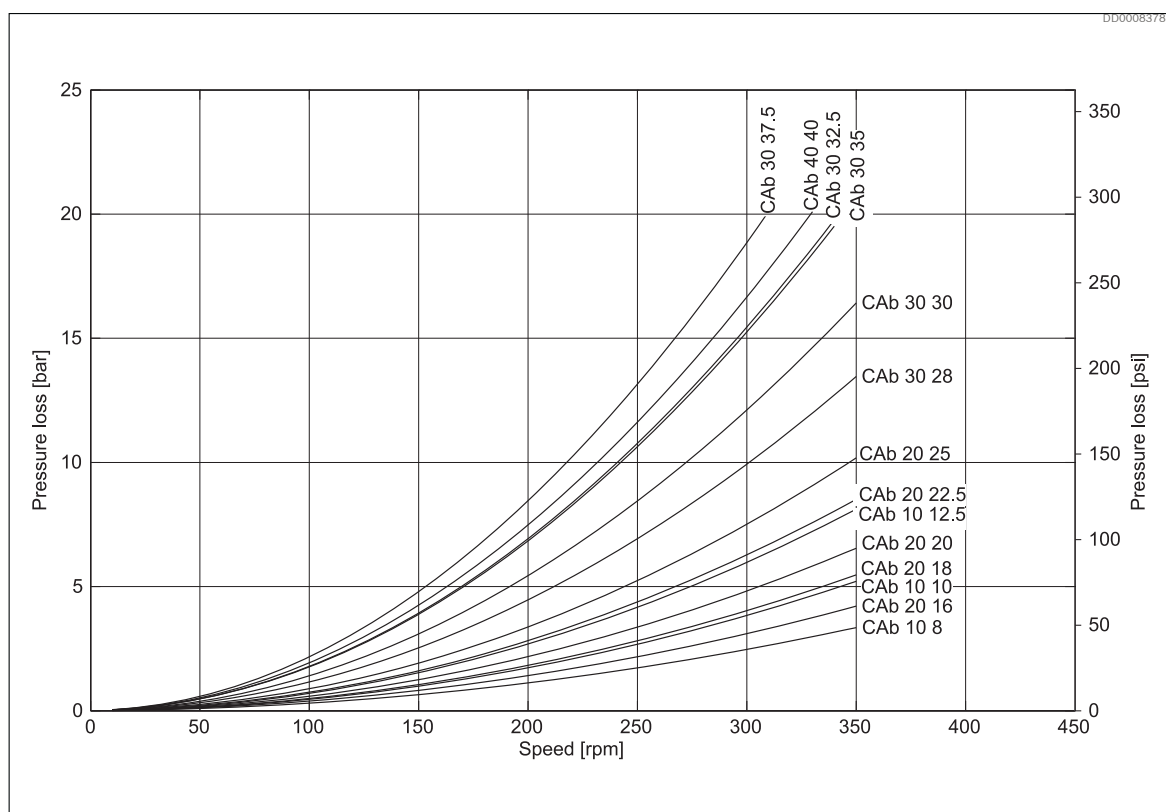
Fig. 22: CAb 10 to CAb 40 pressure loss
