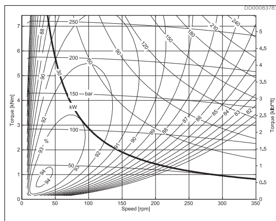
Fig. 17: CAB 30 30, 2 port connection
