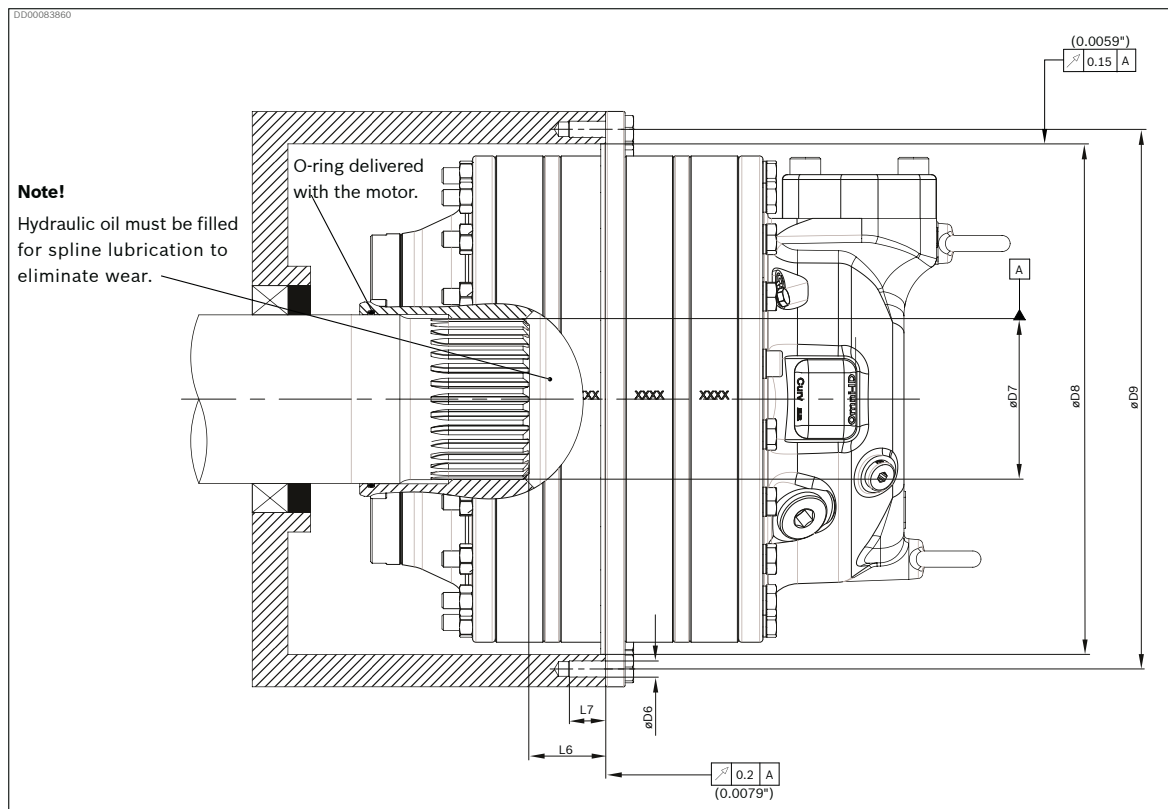
Fig. 48: Shaft installation tolerances CAb 30 C (center flange), CAb 40
