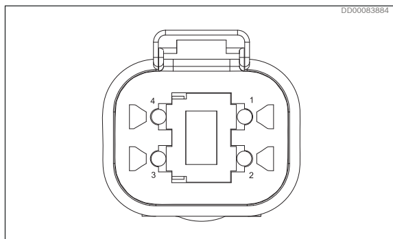
Fig. 50: Mating pin connector
