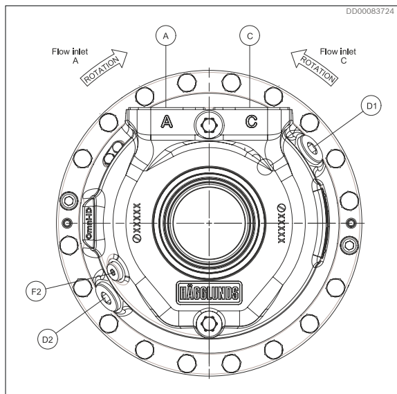
Fig. 3: Connection side of the motor
