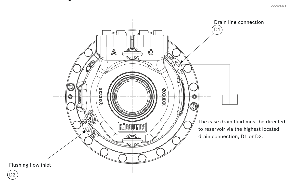
Fig. 24: Horizontal mounting
