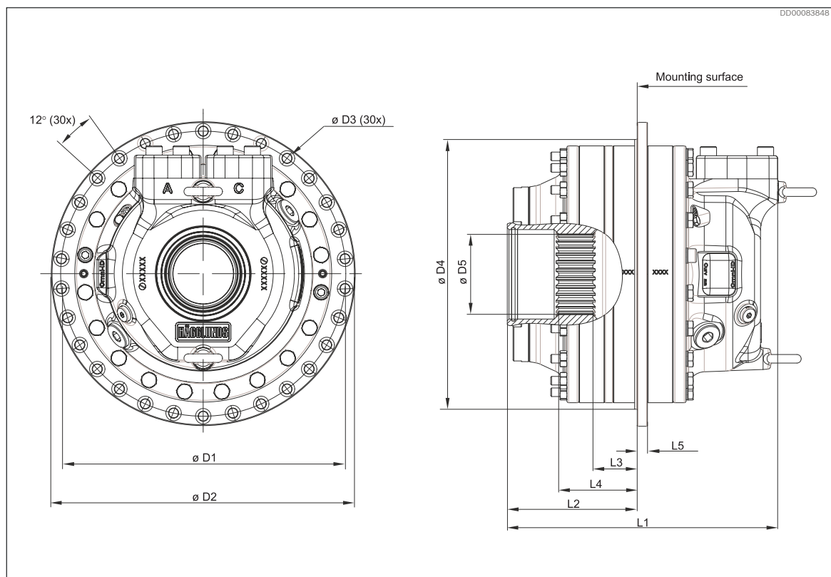
Fig. 45: CAb 30 C (center flange)
