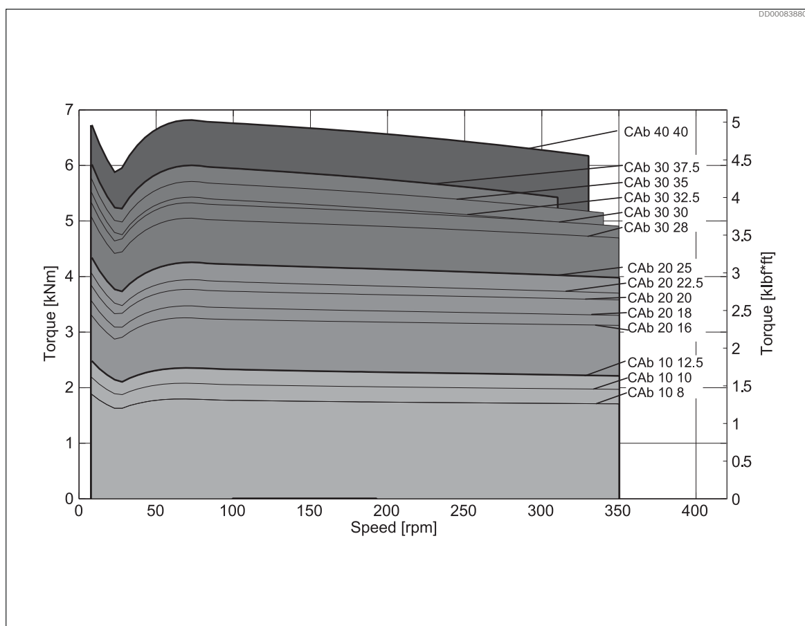
Fig. 23: Quick selection diagram
