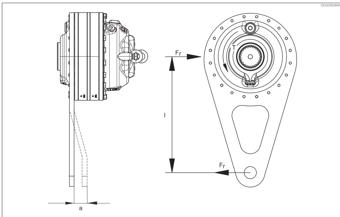
Fig. 30: Shaft mounted motor with torque arm.
