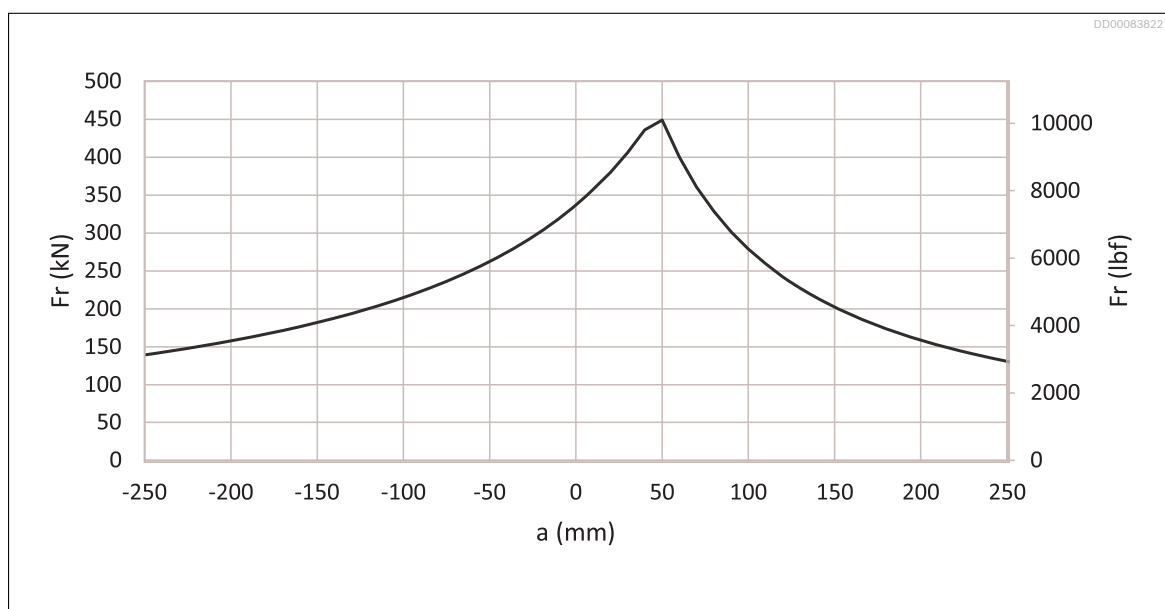
Fig. 39: Permissible external static load Häggglunds CAB 30 28 F and CAB 30 30 F (front flange)
