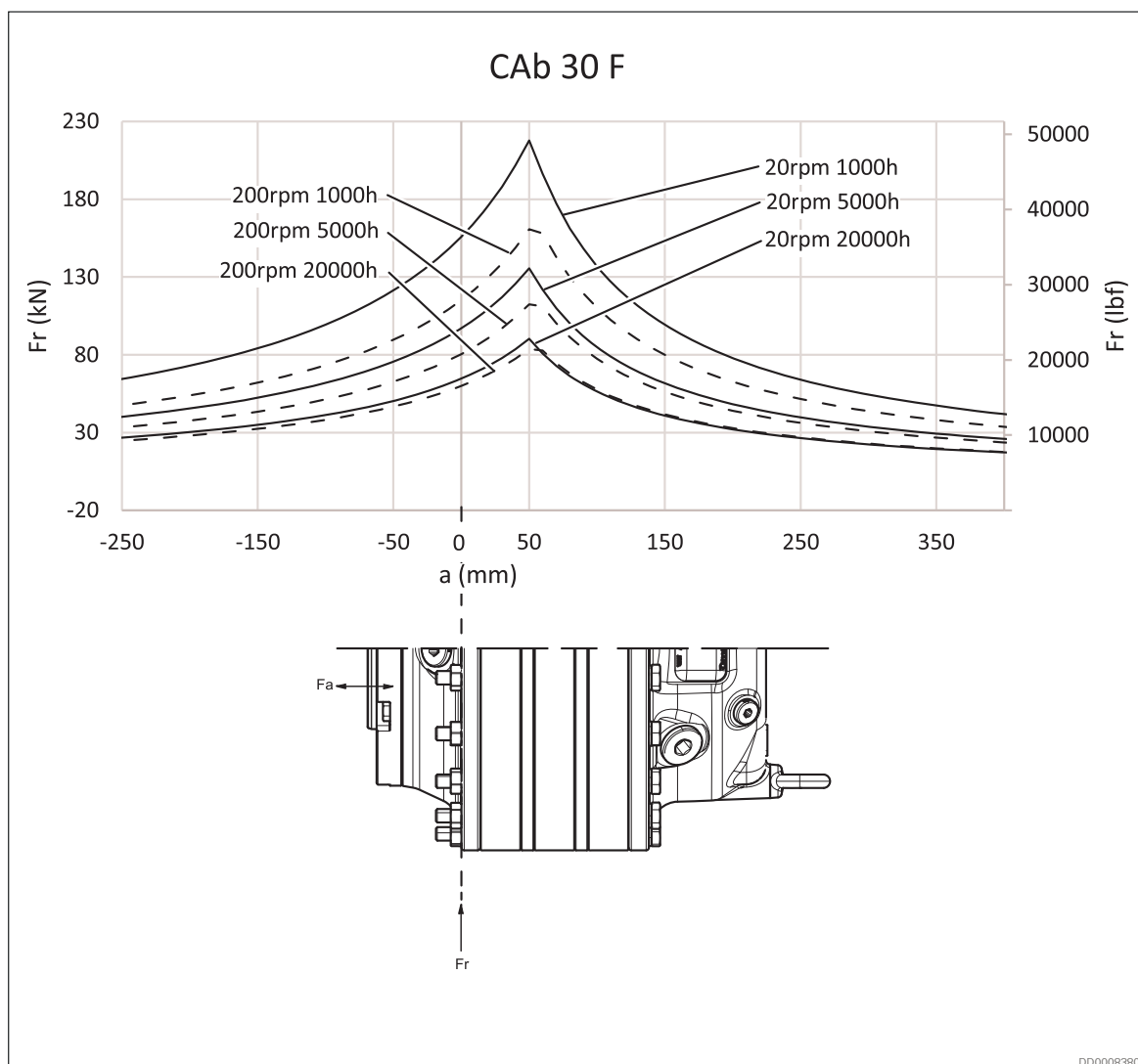
Fig. 34: Permissible external dynamic load Häggblunds CAb 30 28 F and CAb 30 30 F (front flange)
