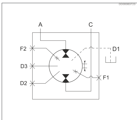
Fig. 2: Hydraulic symbol, radial piston hydraulic motor
