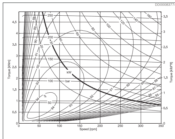
Fig. 13: CAB 20 20, 2 port connection
