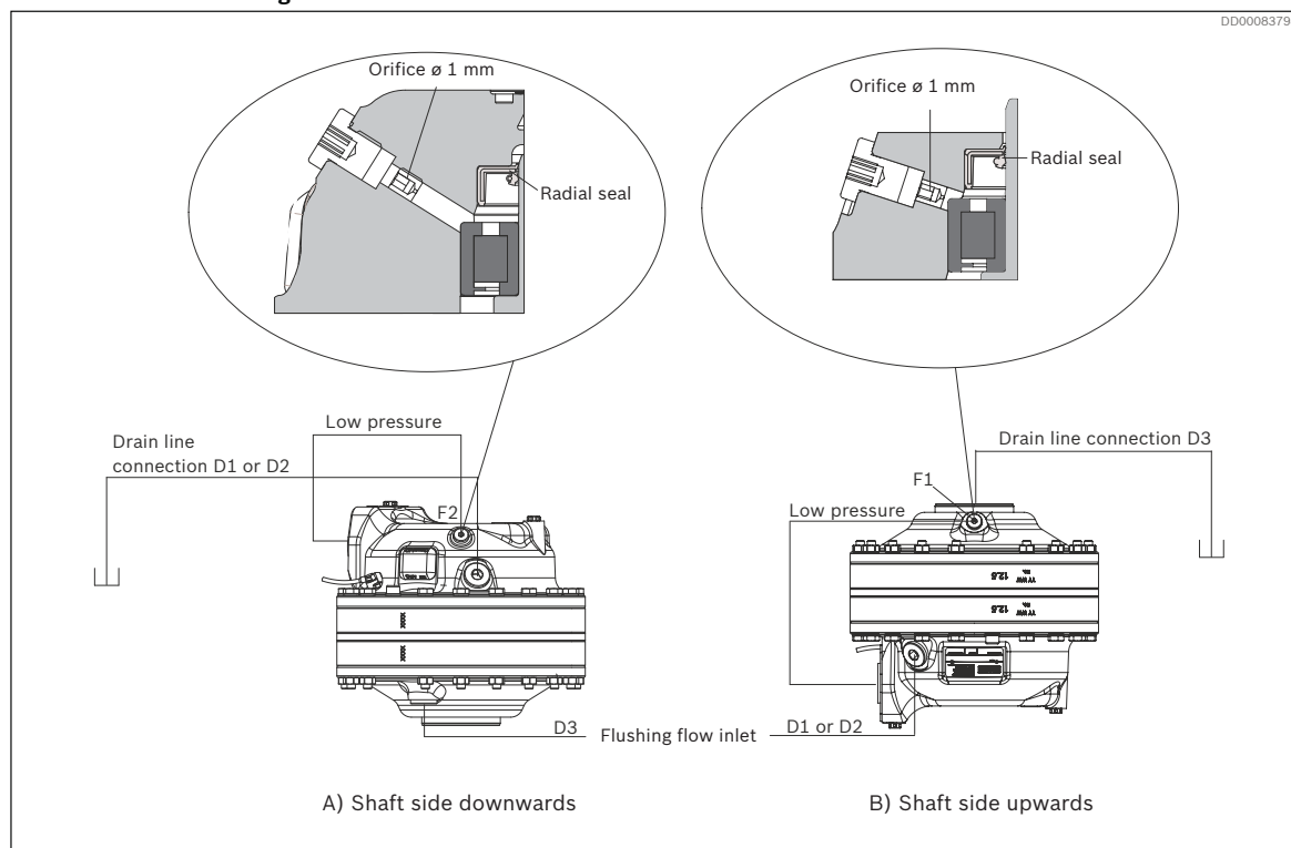
Fig. 25: Vertical mounting
