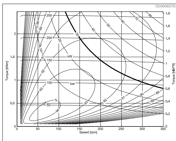
Fig. 9: CAB 10 10, 2 port connection
