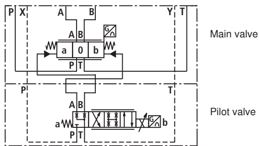
Symbol in detail (external control oil inlet and outlet)
