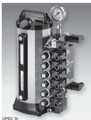
Seat valve modules "S"
