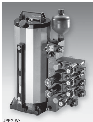
Directional valve module "W"
