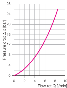
\Delta p -Q characteristic curve for kinematic viscosity of 53 \times 10^{-6} \text{ m}^2/\text{s} (HLP 22 at 20 °C)
