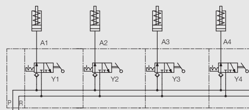
Hydraulic circuit diagram for four circuits with single-acting cylinders
