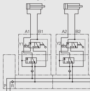
Hydraulic circuit diagram for two double-acting cylinders
